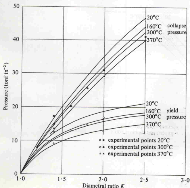
Figure 21. Yield and collapse pressures of Vibrac cylinders calculated from torsion data.
