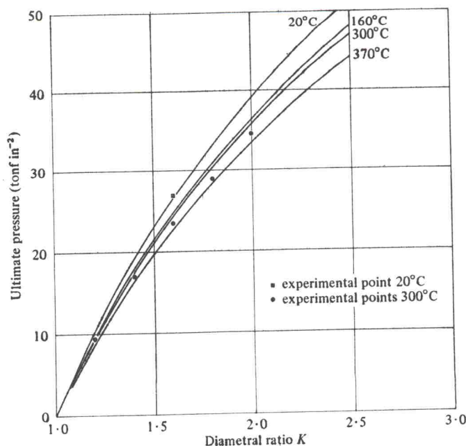
Figure 20. Ultimate pressure of Hykro cylinders calculated from torsion data.
